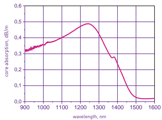
BPDF-SM-8/125-1320
